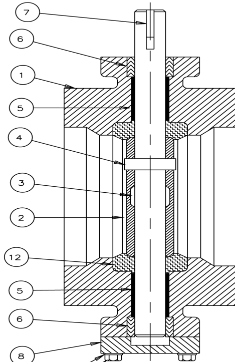
10" THRU 20" 2FI FLANGED & MJE VALVES
