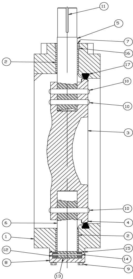
OPTIONAL REPLACEABLE PACKING BONNET ASSEMBLY
